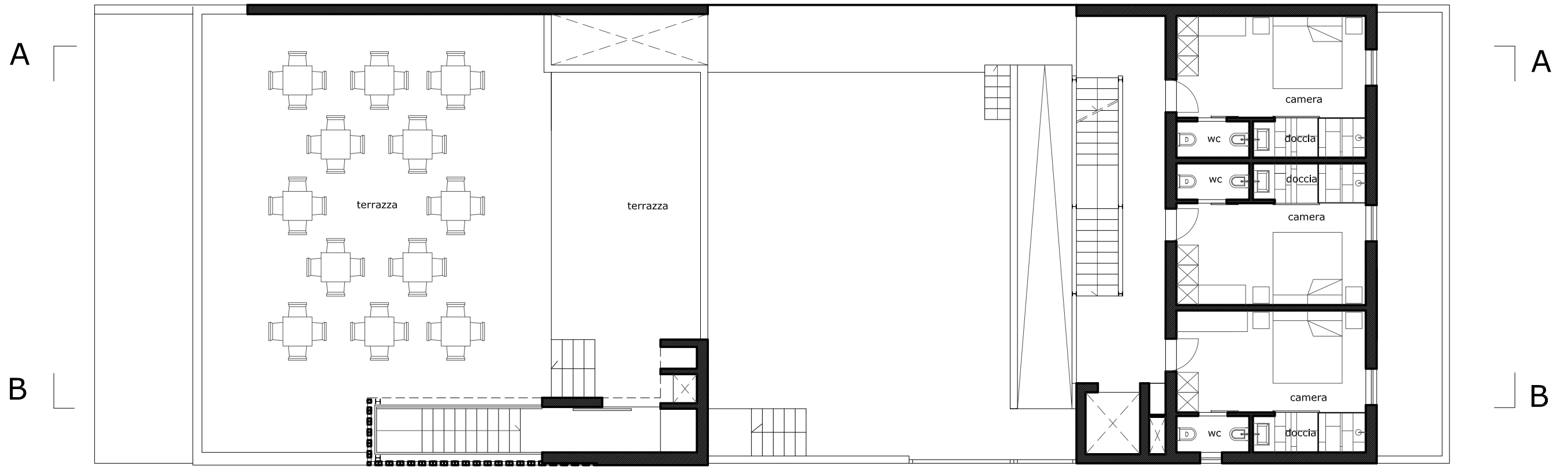
piano terrazza
